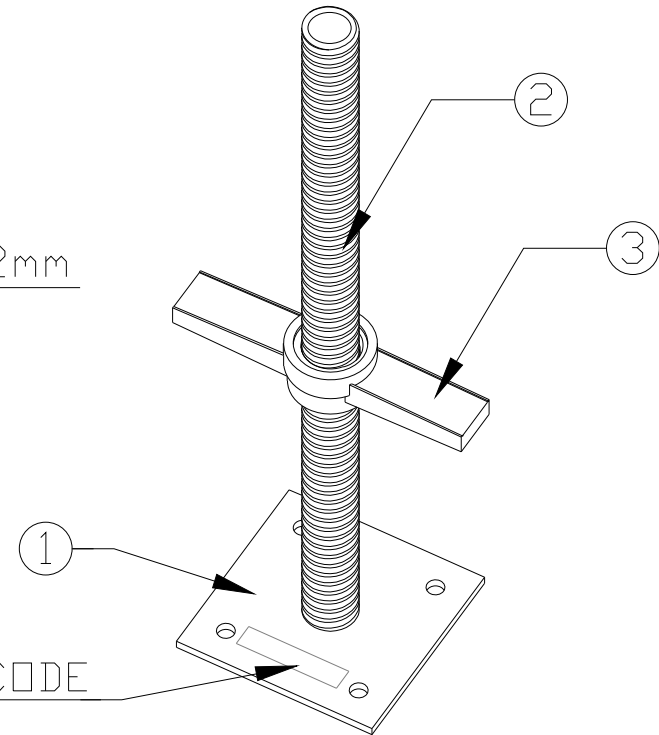
Ø38MM SCREWJACK HOLLOW DIAGRAM
