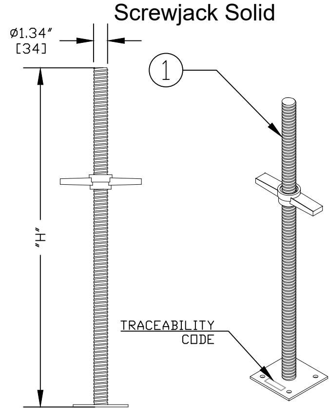
SCREWJACK SOLID DIAGRAM
