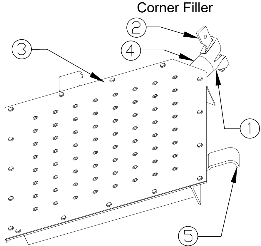
CORNER FILLER DIAGRAM
