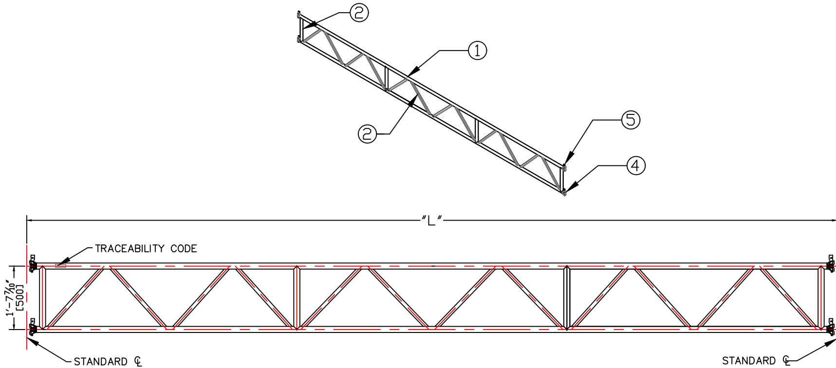
LATTICE GIRDER DIAGRAM
