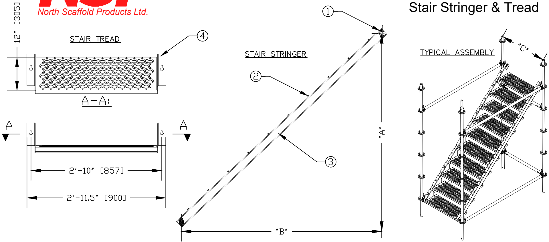
STAIR STRINGER & STAIR TREAD DIAGRAM
