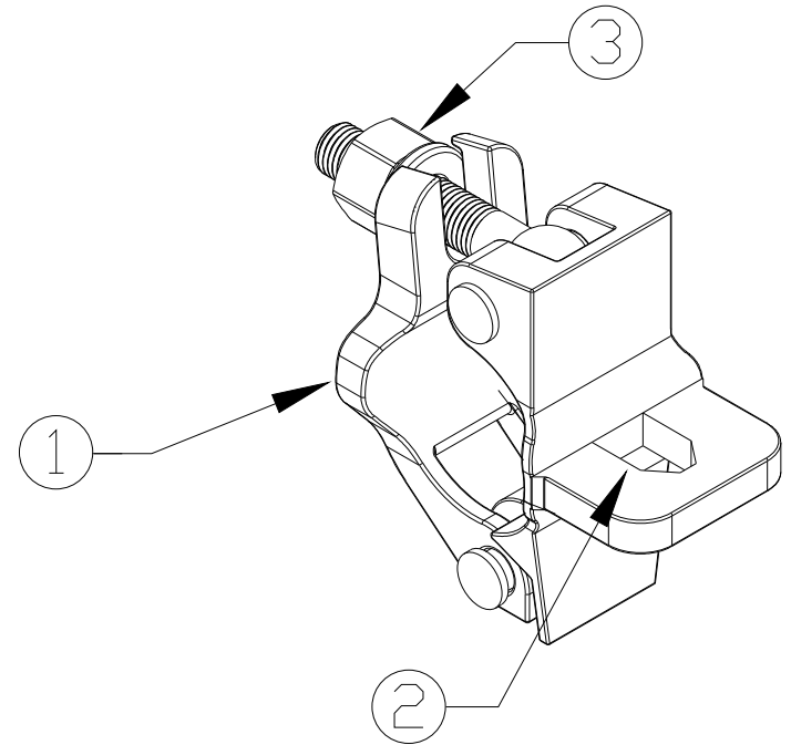
TRANSOM ADAPTOR DIAGRAM
