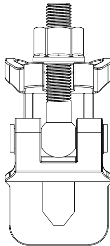
SIDE PROFILE
