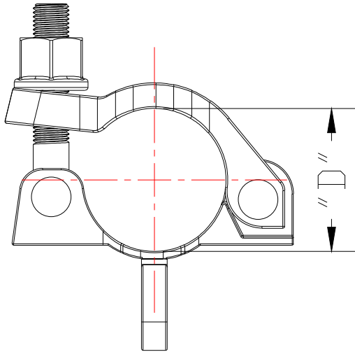
FRONT PROFILE
