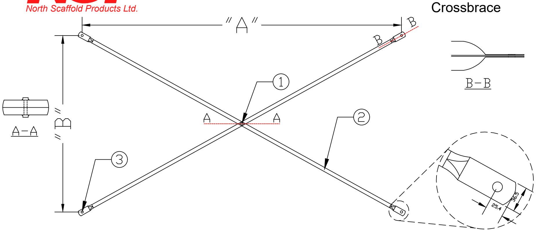
CROSSBRACE DIAGRAM
