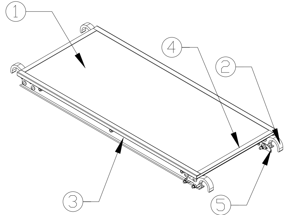
ULTRA LITE™ CFRT DECK DIAGRAM
