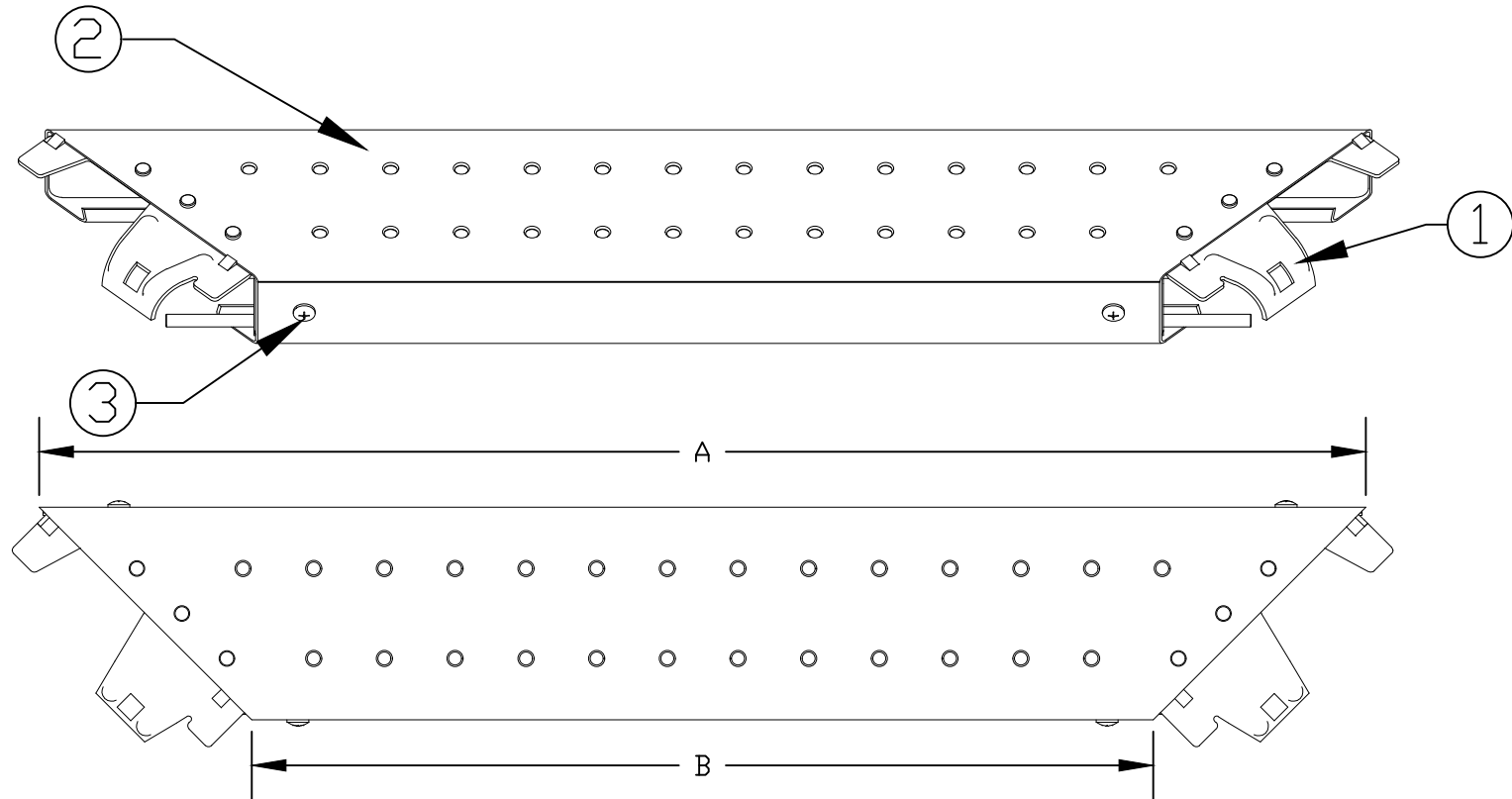
CORNER PLANK DIAGRAM
