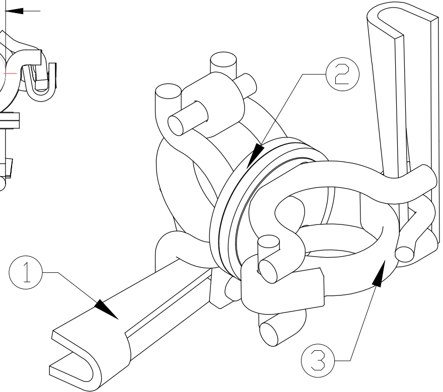
SWIVEL WEDGE CLAMP DIAGRAM
