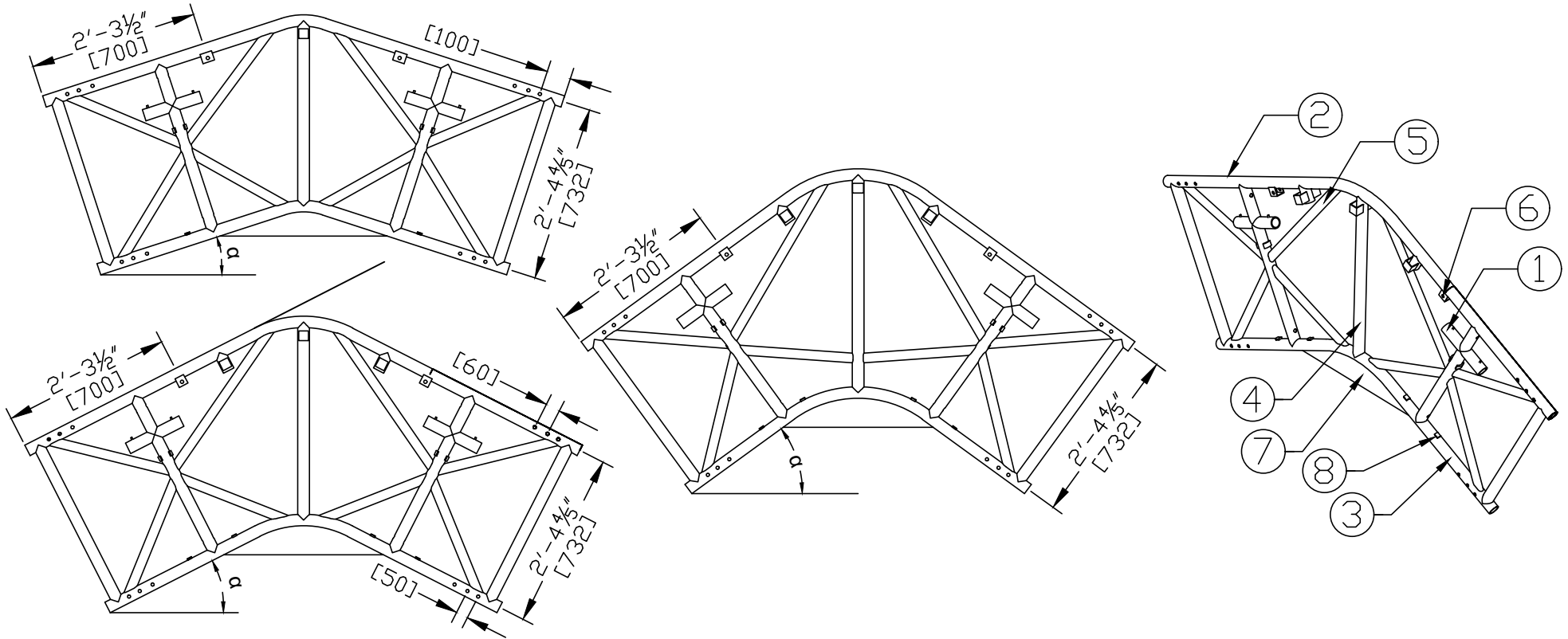
DIAMOND RIDGE BEAM DIAGRAM
