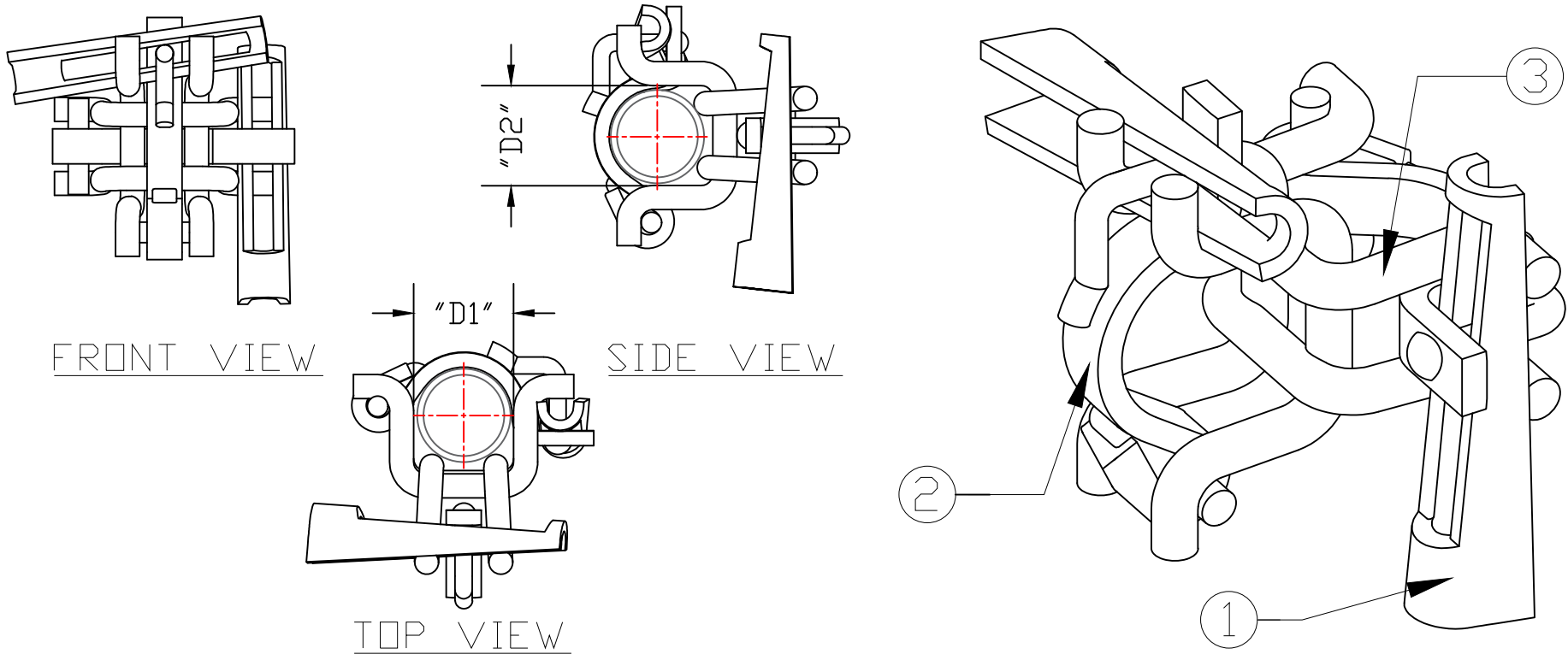
RIGHT ANGLE WEDGE CLAMP DIAGRAM
